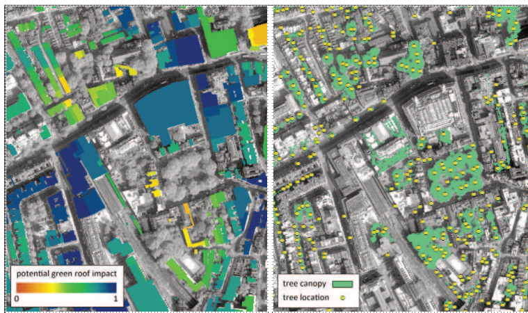
Fig. 2: London – estimated impact of identified potential green roofs (left), tree canopy coverage and tree locations (right) derived for part of the RBKC.
